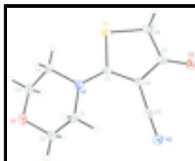
Fig. 1. Molecular structure of the title compound, showing 50% probability displacement ellipsoids and atom numbering scheme. H atoms are drawn as circles with arbitrary small radius.
